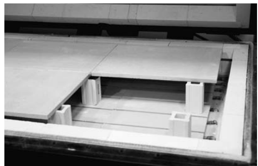
FIGURE 4: POSITIONING THE MULLITE SUBSHEF UNITS.
